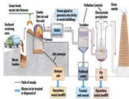
3.4.1.1 Figure 6: Mass burn process, obtained from National Research Council [23].
