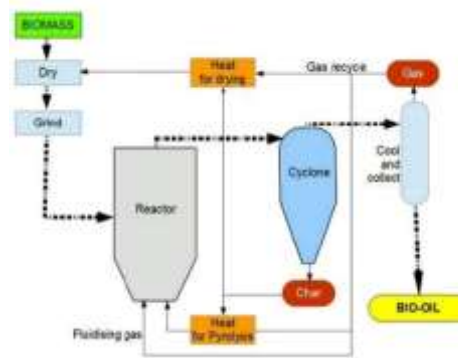
3.2.1.1 Figure 5: Pyrolysis process diagram [18]
